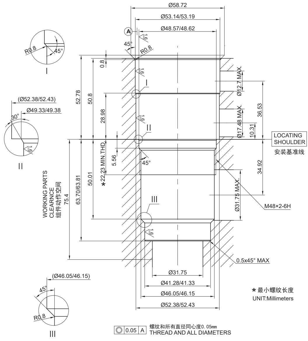
CAVITY: SUN T-24A
