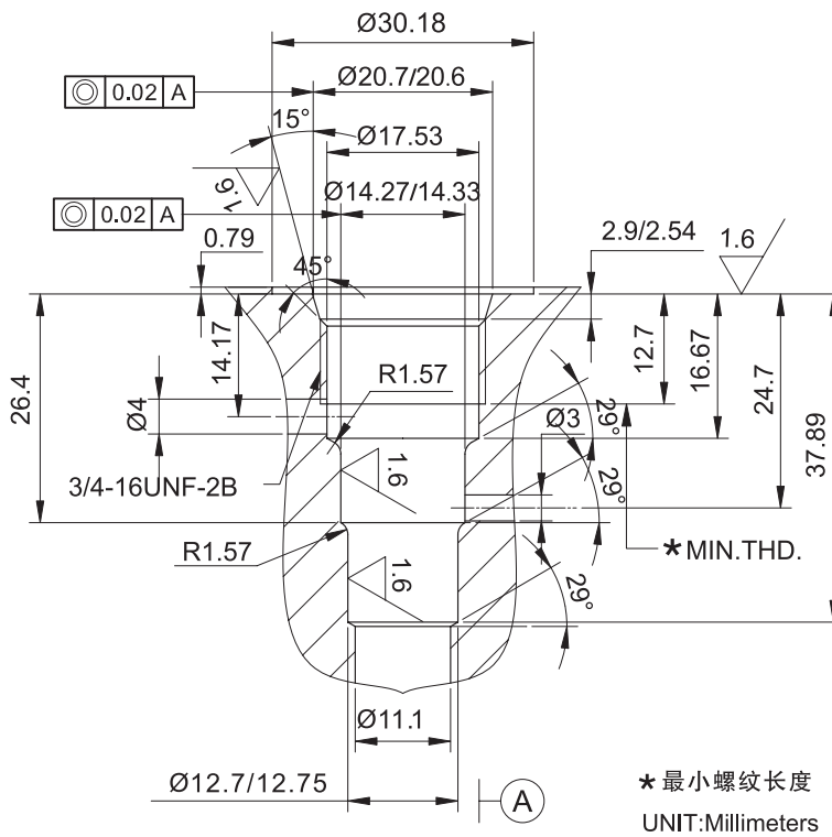
CAVITY: 08-3S
