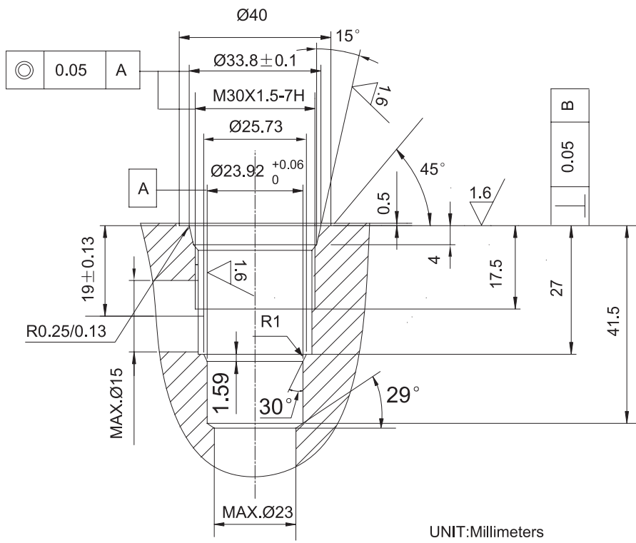
CAVITY: 14M-2
