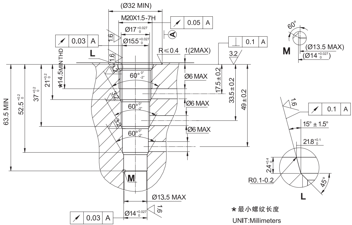
CAVITY: HYDAC 08140
